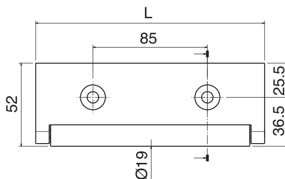
TYPE B - WITH ROLLER BEARING
